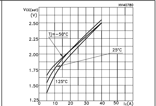
Figure 9. Collector-emitter on voltage vs collector current
